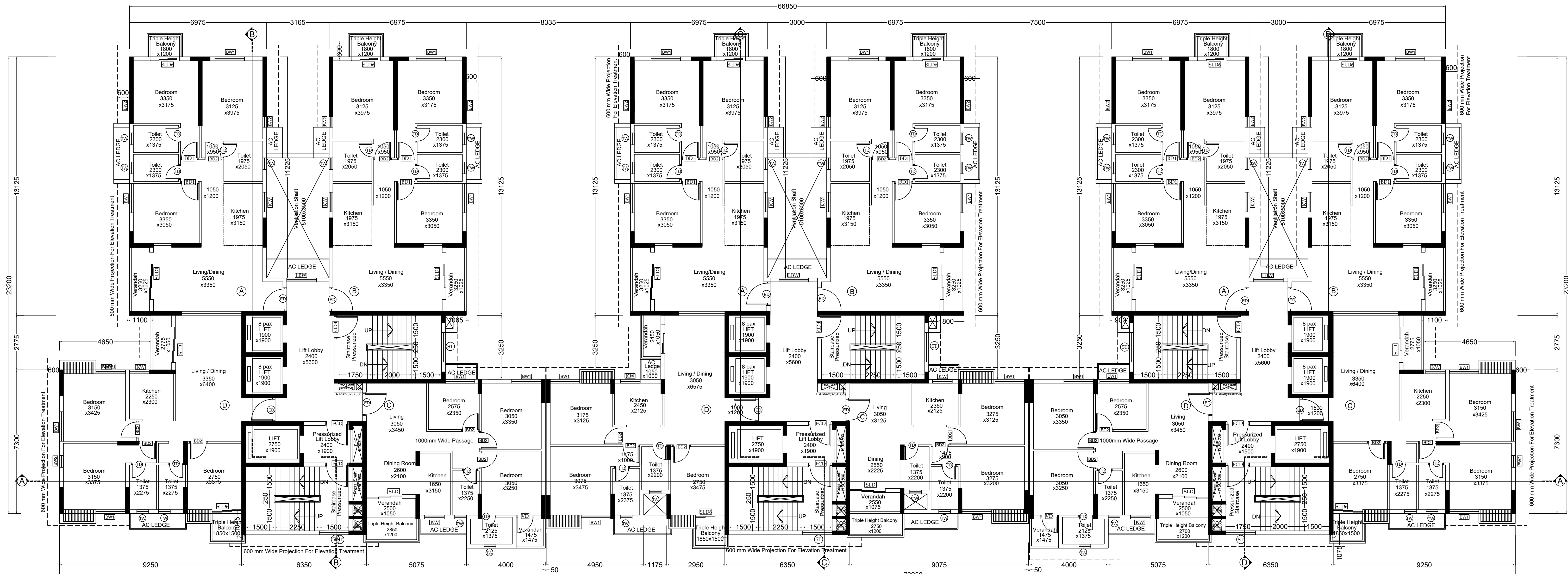
BLOCK-1 WING-A
